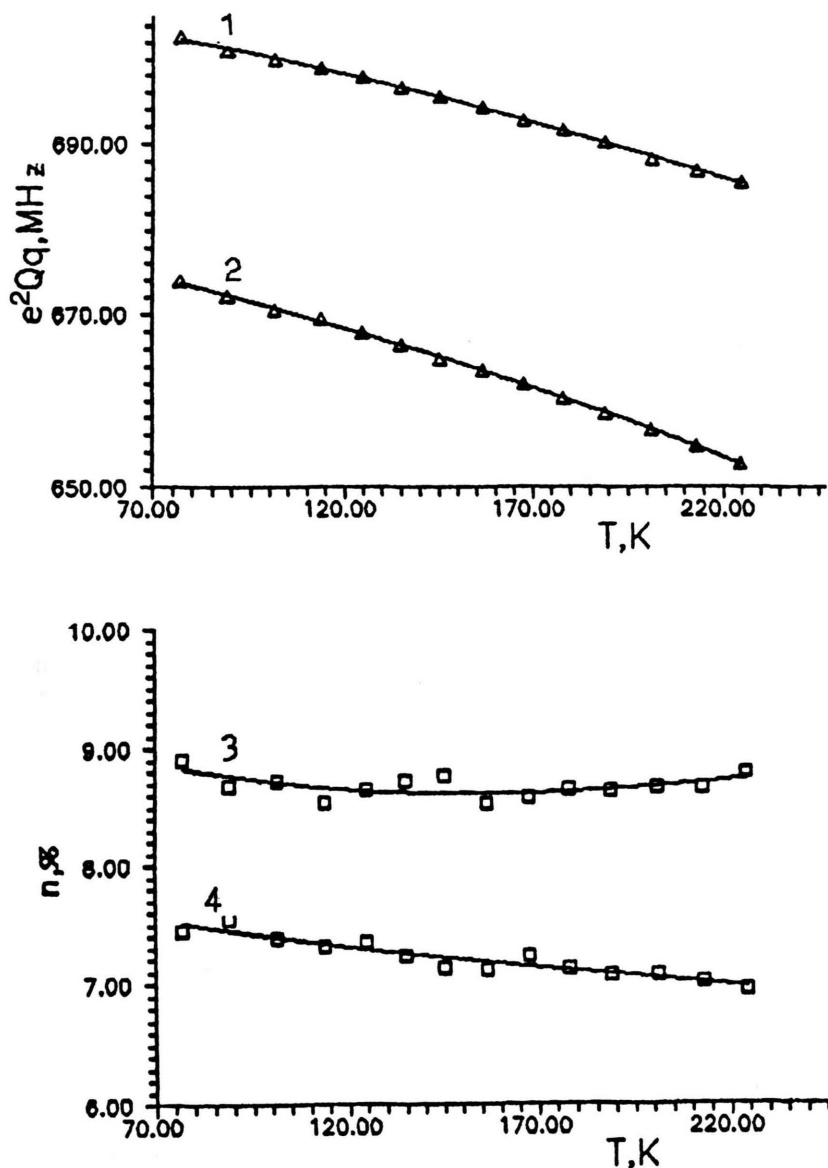
Fig. 3. Temperature dependence of the quadrupole coupling constants e^2Qq (1 and 2 for Sb_1 and Sb_2 ) and asymmetry parameters \eta (3 and 4 for Sb_1 and Sb_2 ) for the antimony atoms ^{123}\text{Sb} in \text{KSb}_2\text{F}_7 .
